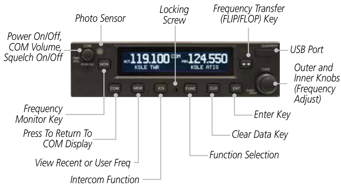
GTR 225 Front Panel Description
